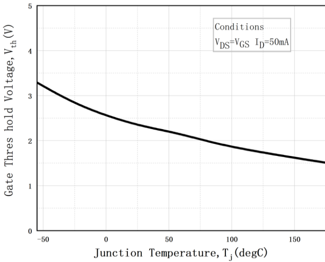
Figure 15. Threshold voltage vs.temperature
